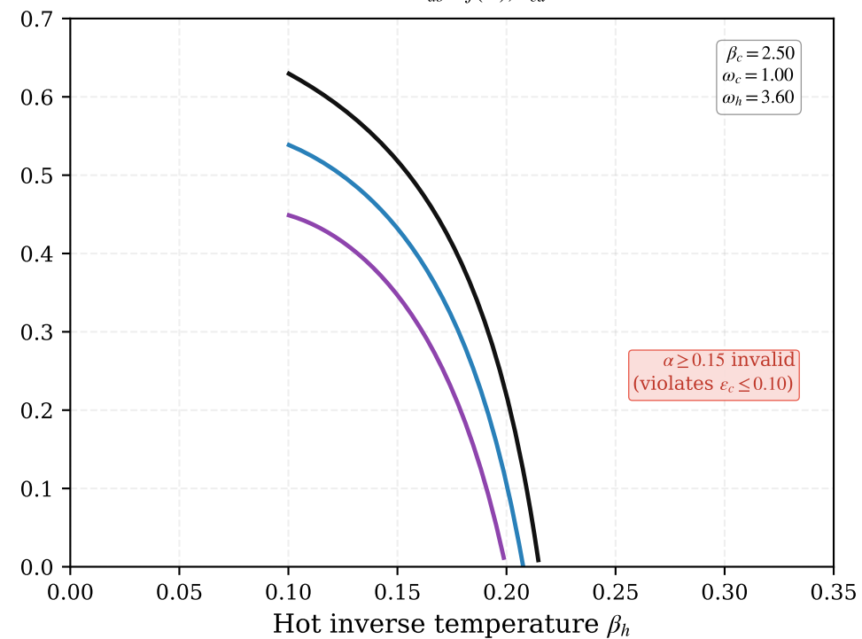
Case 4: \lambda_{ab} = \lambda_{cd} = f(\omega)
